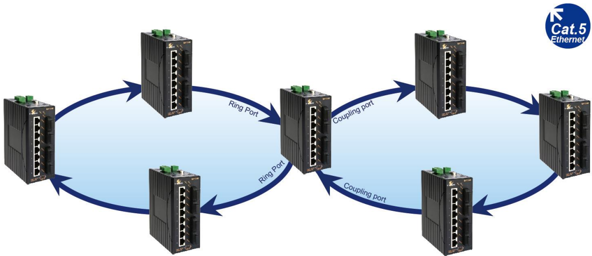
Figure 75: Ring Coupling Example
