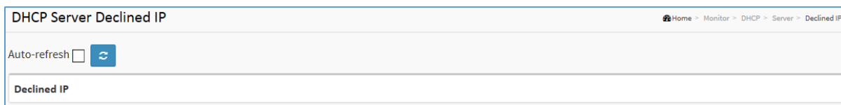
Figure 3-4.1.3: Declined IP
