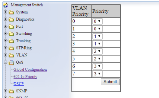
Figure 81: 802.1p Priority
