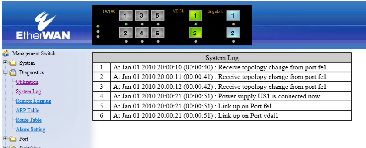
Figure 15: System Log
