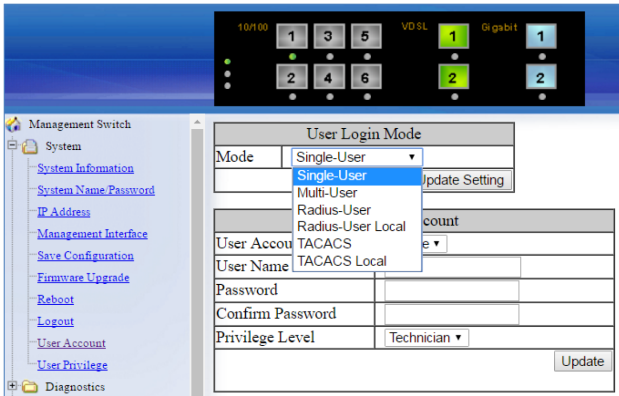
Figure 9: User Mode
