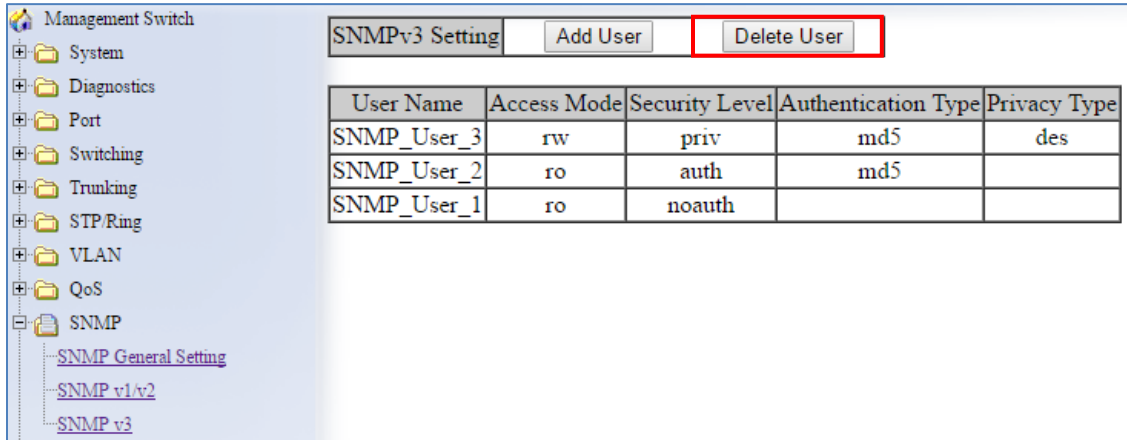
Figure 90: Delete User
