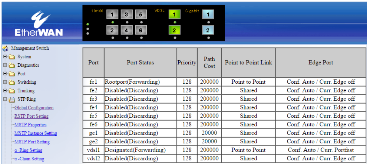
Figure 47: Spanning Tree Port Roles
