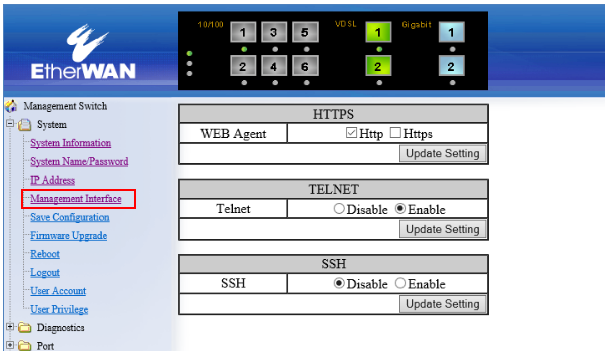
Figure 6: Management Interface
