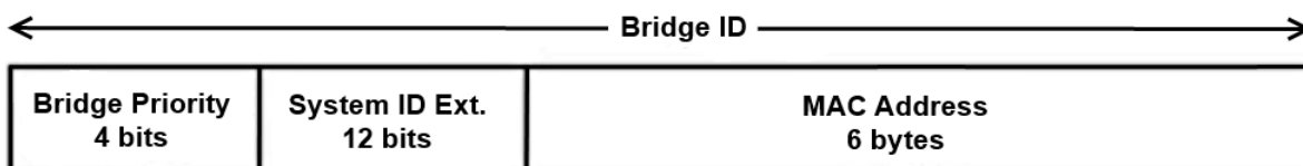
Figure 60: Bridge ID
