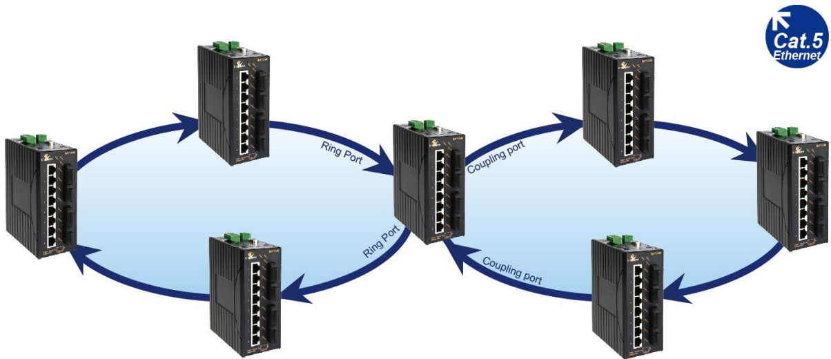
Figure 73: Ring Coupling Example
